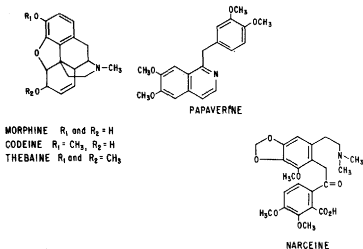
Fig. 1. Structural formulae of Papaver somniferum alkaloids.
